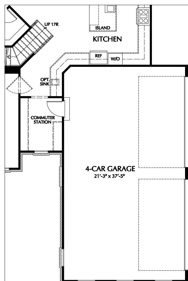
PARTIAL FIRST FLOOR PLAN - OPTIONAL 4-CAR GARAGE
