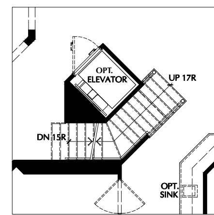
PARTIAL FIRST FLOOR PLAN - OPTIONAL ELEVATOR CONDITION
