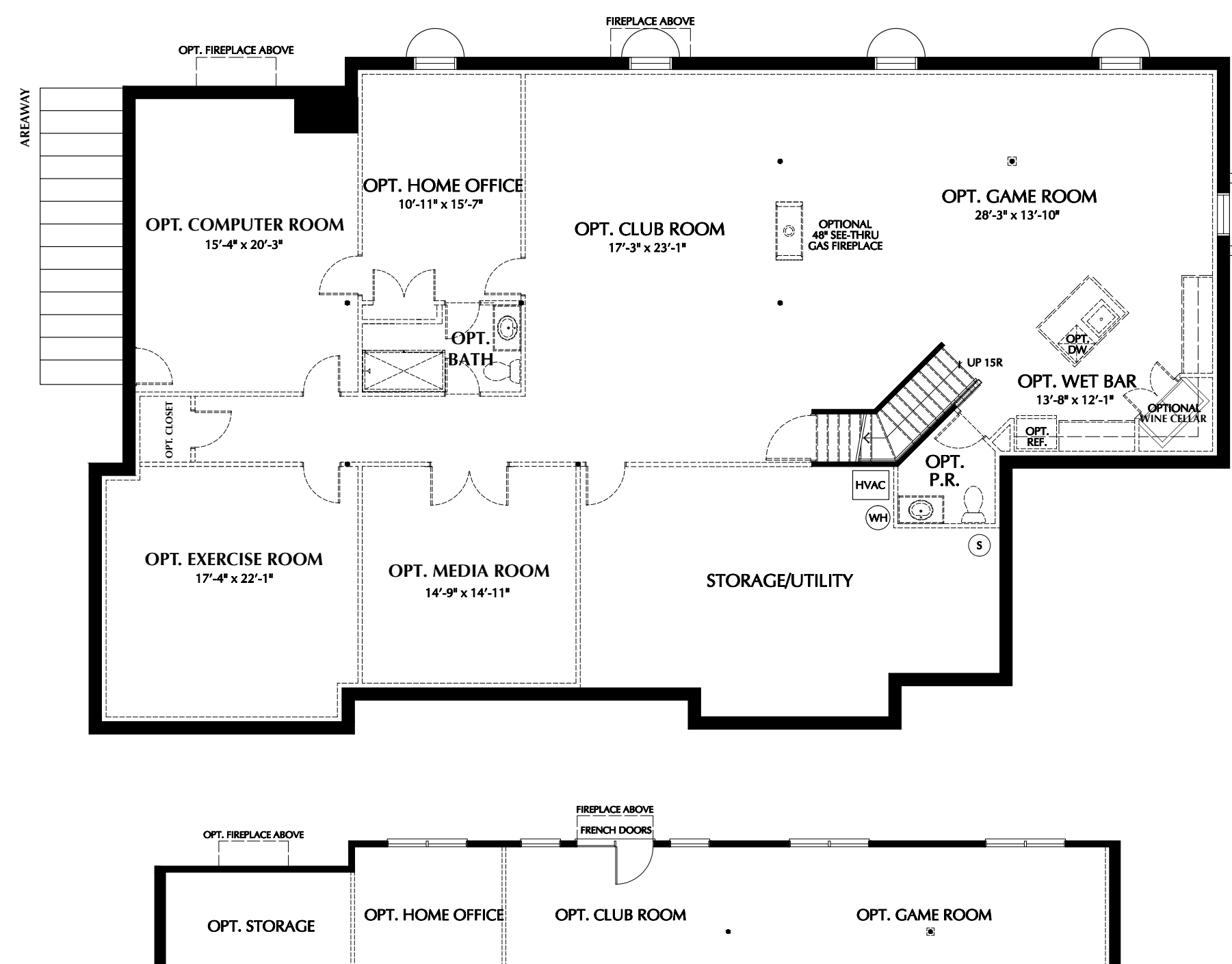
PARTIAL BASEMENT PLAN w/ALTERNATE WALKOUT CONDITION
