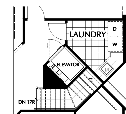
PARTIAL SECOND FLOOR PLAN - OPTIONAL ELEVATOR CONDITION
