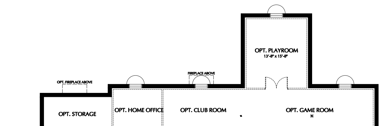
PARTIAL BASEMENT PLAN - OPTIONAL REAR SUNROOM OR SCREEN PORCH ABOVE
