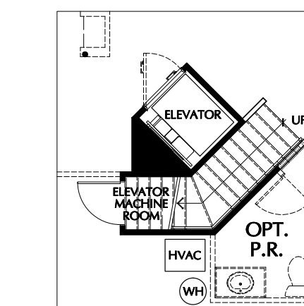
PARTIAL BASEMENT PLAN - OPTIONAL ELEVATOR CONDITION
