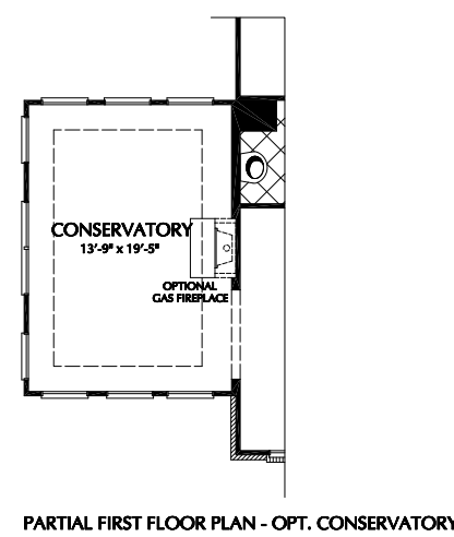
PARTIAL FIRST FLOOR PLAN - OPT. CONSERVATORY
