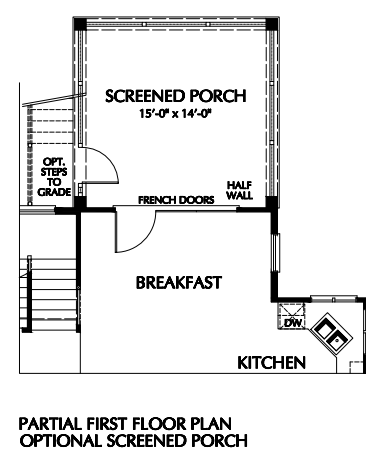
PARTIAL FIRST FLOOR PLAN OPTIONAL SCREENED PORCH
