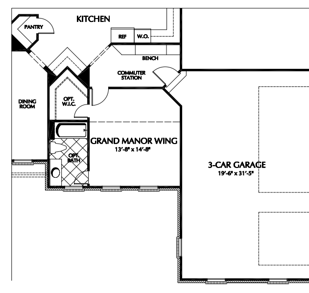
PARTIAL FIRST FLOOR PLAN W/ ALT. GRAND MANOR WING
