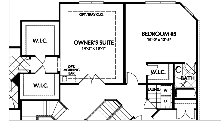
PARTIAL SECOND FLOOR PLAN OPTIONAL FIFTH BEDROOM
