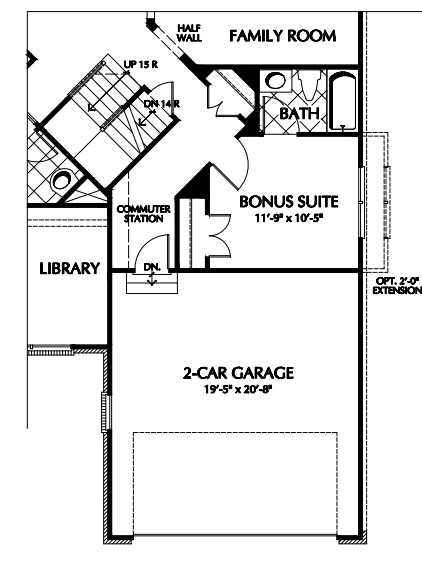
PART. FIRST FLOOR PLAN OPTIONAL BONUS SUITE
