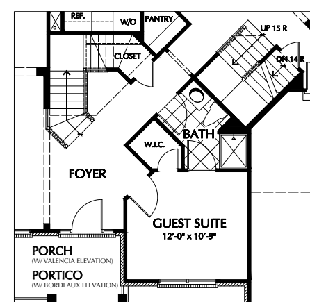
PART. FIRST FLOOR PLAN OPTIONAL GUEST SUITE
