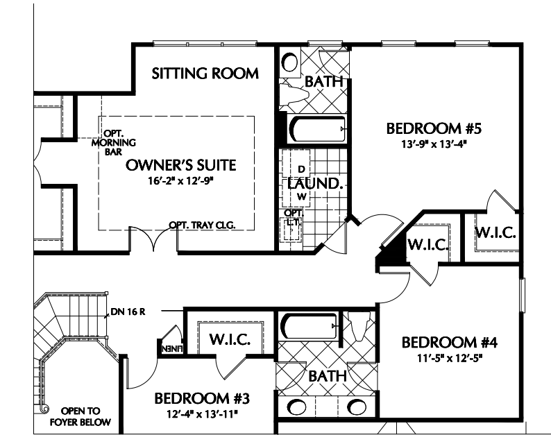
PARTIAL SECOND FLOOR PLAN OPTIONAL FIFTH BEDROOM
