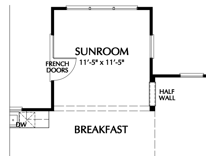
PARTIAL FIRST SECOND FLOOR PLAN OPTIONAL SUNROOM
