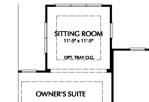
PARTIAL SECOND FLOOR PLAN OPTIONAL SUNROOM
