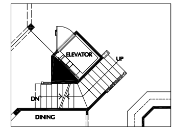
PARTIAL FIRST FLOOR PLAN W/ OPT. ELEVATOR
