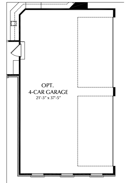
PARTIAL FIRST FLOOR PLAN - OPT. 4-CAR GARAGE (PER ELEVATION)
