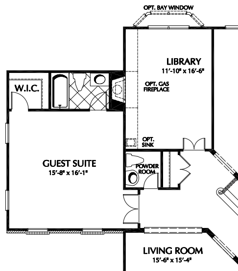
PARTIAL FIRST FLOOR PLAN - OPTIONAL GUEST SUITE
