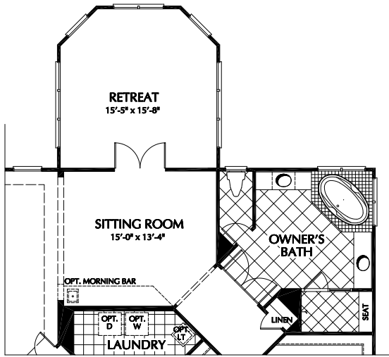
PARTIAL SECOND FLOOR PLAN - OPTIONAL RETREAT
