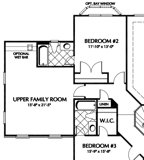
PARTIAL SECOND FLOOR PLAN - OPTIONAL UPPER FAMILY ROOM
