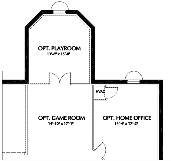
PARTIAL BASEMENT PLAN - OPTIONAL REAR SUNROOM
