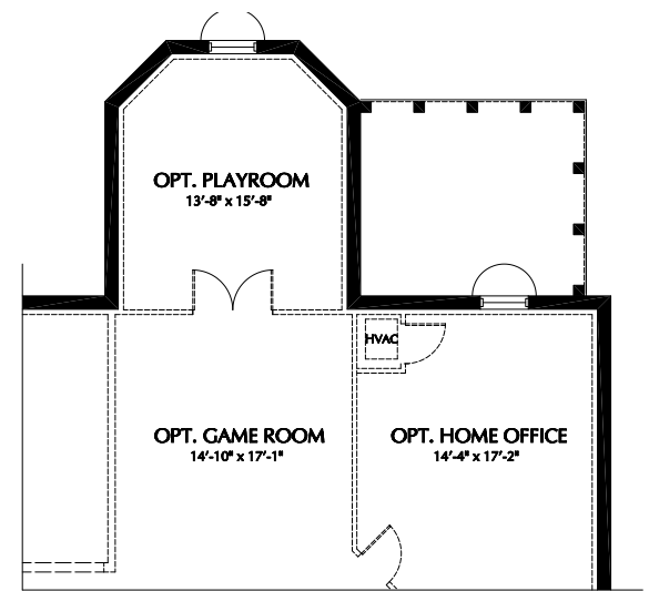
PARTIAL BASEMENT PLAN - OPT. REAR SUNROOM/SCREENED PORCH
