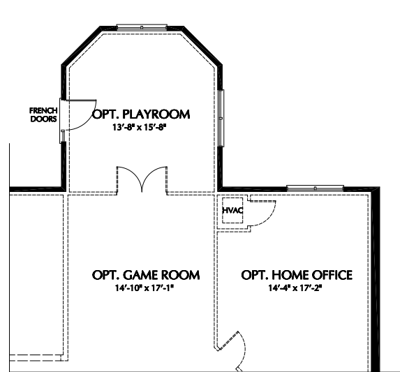
PARTIAL BASEMENT PLAN - OPT. REAR SUNROOM w/WALKOUT CONE
