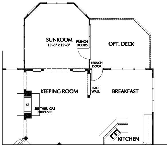
PARTIAL FIRST FLOOR PLAN - OPTIONAL REAR SUNROOM
