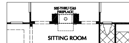
PARTIAL SECOND FLOOR PLAN - OPT. FIREPLACE
