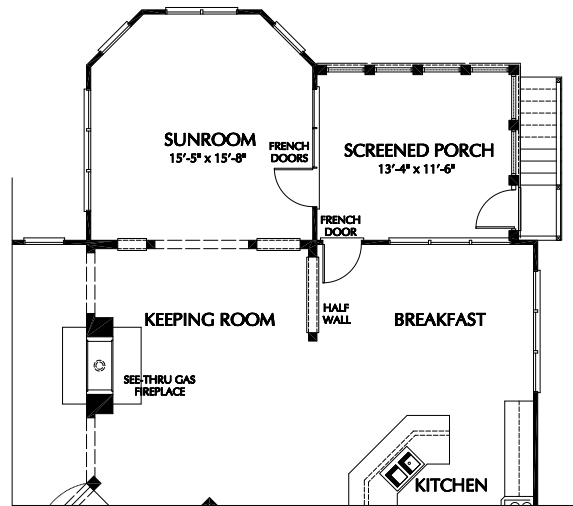
PARTIAL FIRST FLOOR PLAN - OPT. REAR SUNROOM/SCREENED PORCH
