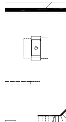
PARTIAL BASEMENT PLAN w/OPT. FIREPLACE - SINGLE OR DOUBLE SIDED
